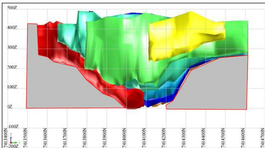
Figure 1: Schematic cross section of Kallak North
